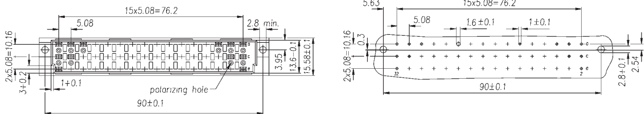
Printed Circuit Layout
