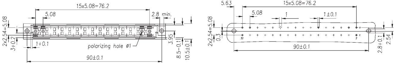
Printed Circuit Layout
